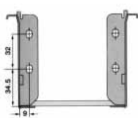
前連接件安裝尺寸 Front connector mounting dimensions
