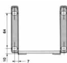
背板安裝尺寸 Back panel mounting dimensions
